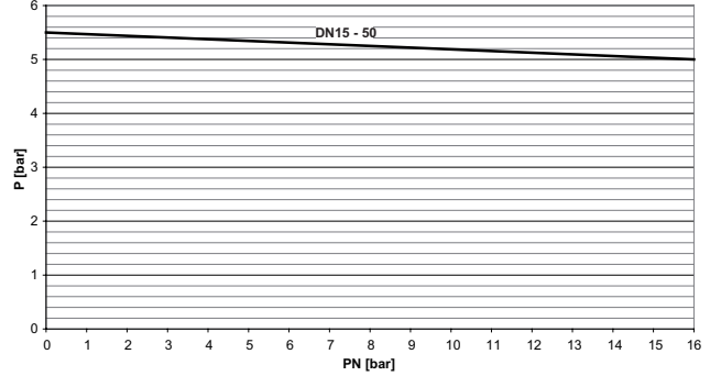
DIASTAR SIXTEEN, FC with PTFE diaphragm
